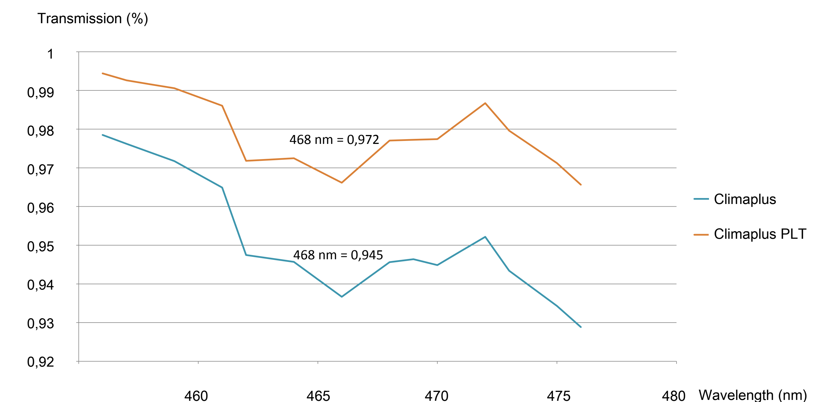
Fig. II. Two glasstypes and their different transmittance of the full spectrum light is tested in this study 1 = 2-layered low-iron glass 2 = 3-layered float glass NB. The figure shows spectral transmittance in the sensitive area of IpRGCs 460 – 480 nm
