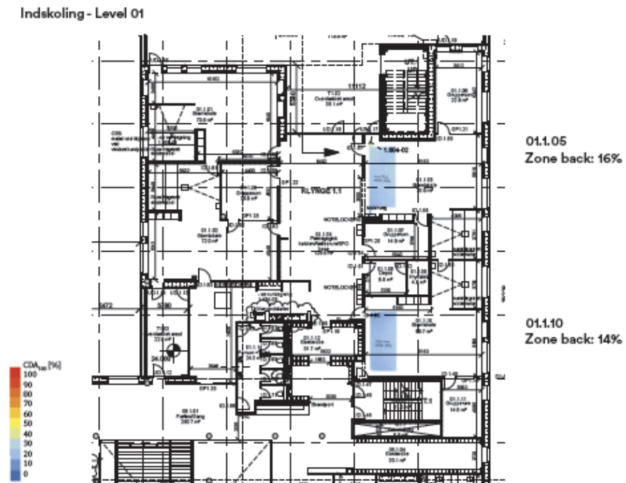
Figure 6.25: Daylight simulation level 01.
