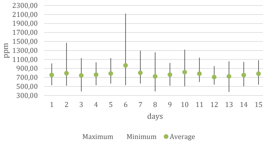
Figure 6.16: CO 2 concentration, first 15 test days
