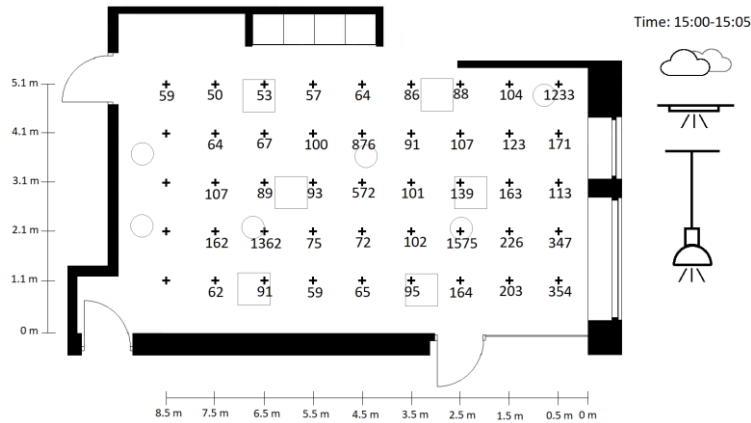
Room 1.1.10 New Scenario B – Ambient CL (30%) + Focussed Pendants (100%) daylight-hours.
