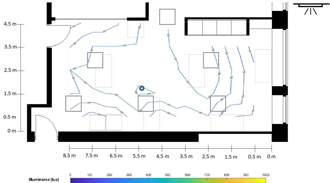
Figure 6.4: Illuminance levels [lux] at 0.6m above floor level in room 1.2.10 under New Scenario A - Ambient Ceiling Lighting (70% output) for electric lighting only.
