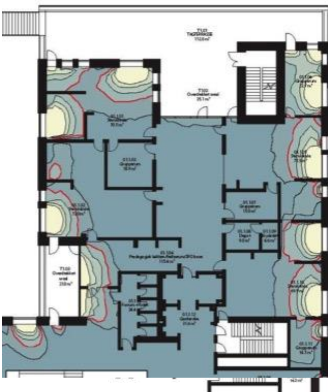
Daylight factor _ CLASSROOM 1A + 1B
