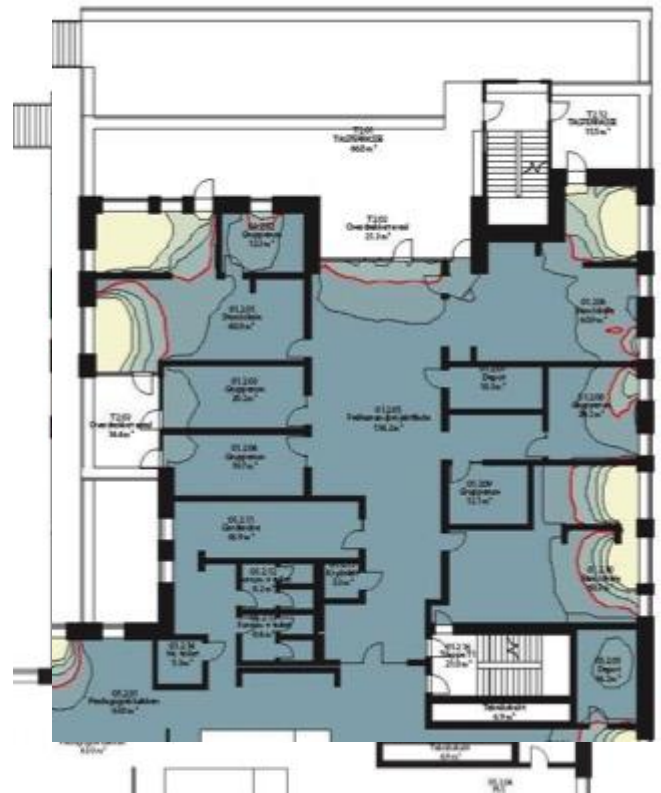
Daylight factor _ CLASSROOM 2A + 2B
